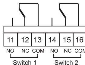
Micro switches 1, 2
