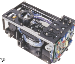
Torque Switch
