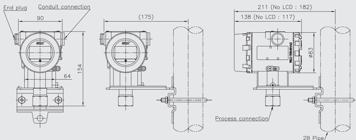
2" MOUNTING TYPE
