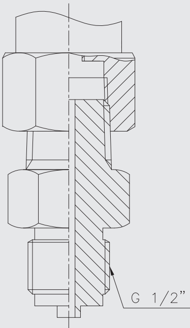
G1/2 male thread
